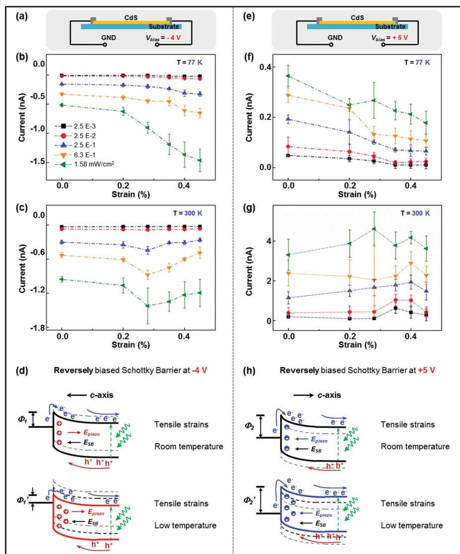
Figure 4. Temperature dependence of the piezophototronic effect and the working mechanism. a) At a bias voltage of -4 V, the current I versus strains curve under a series of illumination intensities at b) 77 K and c) 300 K, and d) the corresponding energy band diagrams of CdS NWs under tensile strains at room temperature (top panel) and low temperature (bottom panel). e) At a bias voltage of +5 V, the current I versus strains curve under a series of illumination intensities at f) 77 and g) 300 K, and h) the corresponding energy band diagrams of CdS NWs under tensile strains at room temperature (top panel) and low temperature (bottom panel). The figure legends presented in (b) are adopted for plots in (c), (f), and (g).
