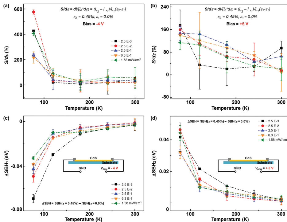
Figure 5. Temperature dependence of the piezophototronic factor at a) -4 and b) +5 V biased voltage. The piezophototronic factor is defined as the response sensitivity per unit strains: S/d\epsilon . The figure legends presented in (a) are adopted for plots in (b). Calculated changes of SBH as a function of temperatures at the reversely biased Schottky contact under c) -4 V and d) +5 V between 0.45\% tensile strain and strain-free condition.
