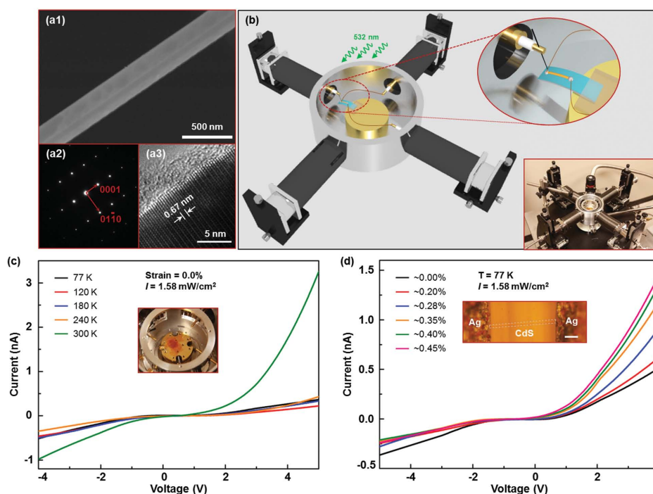
Figure 1. Structure and transport characterizations of CdS NWs. a1) SEM image, a2) SAED pattern, and a3) HRTEM image of the as-synthesized CdS NW. b) Schematic illustration and digital image of the micromanipulation cryogenic probe station system as experimental setups. I – V characteristics of CdS NW devices under various c) temperatures and d) straining conditions.
