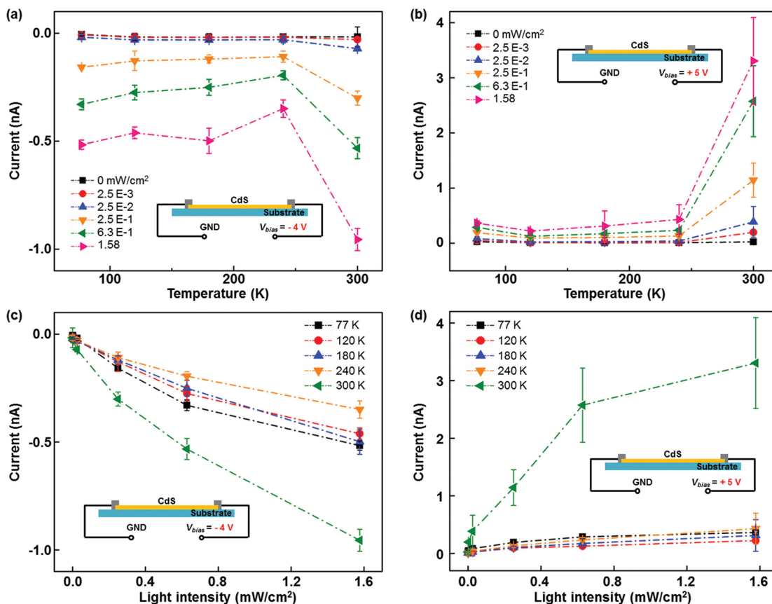
Figure 2. Current response of CdS NW devices to temperatures and illuminations. Current response of CdS NW devices to various temperatures under a series of illumination intensities and strain-free condition at a) -4 and b) +5 \text{ V} biased voltage. Current response of CdS NW devices to various illuminations at different temperatures and under strain-free condition by applying a bias voltage of c) -4 and d) +5 \text{ V} .
