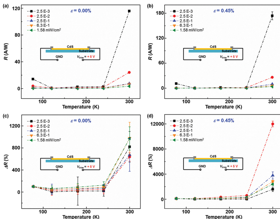
Figure 3. Temperature dependence of the photoresponsivity. Photoresponsivity of the device under various illuminations and temperatures, by applying a) 0.00% and b) 0.45% strain, biased at +5 V. Relative changes of the photoresponsivity under various illuminations and temperatures, by applying c) 0.00% and d) 0.45% strain, biased at +5 V.
